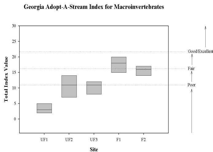
Figure 1. Box plots for Georgia Adopt-A-Stream macroinvertebrate index values and ratings for water quality at each site from February 2002 to February 2003 (median, 25 th and 75 th percentiles, maximum value, minimum value and outliers).
